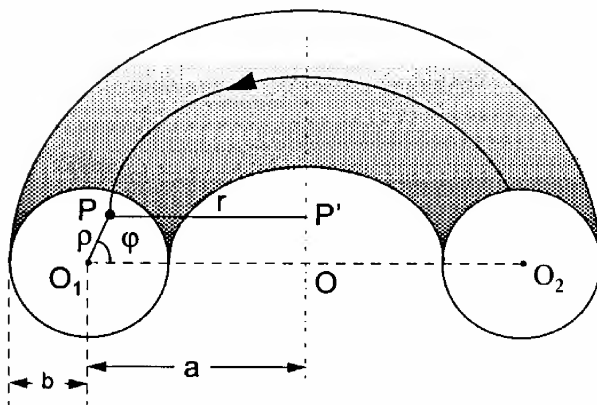
Figura 9.15 Bobina toroidal
