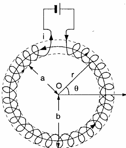
Figura 8.20 Bobina toroidal
